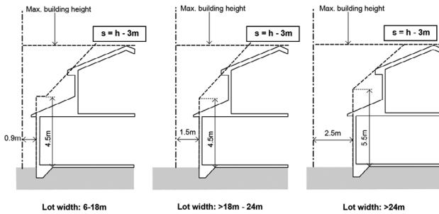
Setback above 4.5m = Building height at any point - 3m (subject to 3C.21(7))
